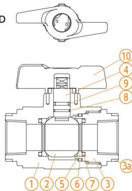
THREADED
